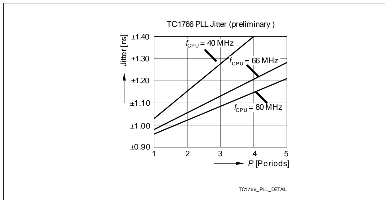
Figure 4-13 Approximated Maximum Accumulated PLL Jitter for Typical CPU Clock Frequencies f_{\text{CPU}} (detail)
